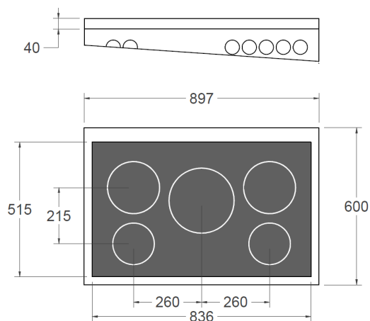
WORKTOP DETAILS
